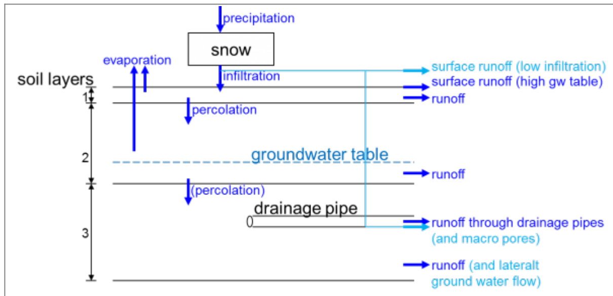
Figure 5: Illustration of flowpaths in the soil in the HYPE model.
