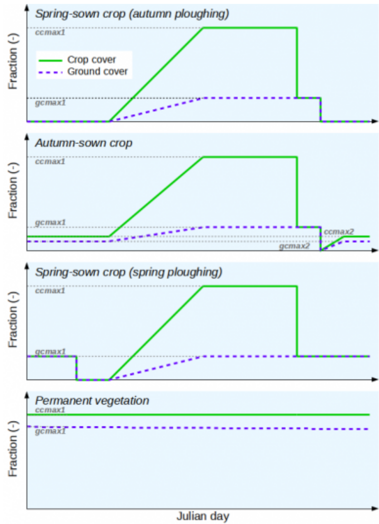
Figure 3: Crop cover and ground cover development for four different crop configurations.
