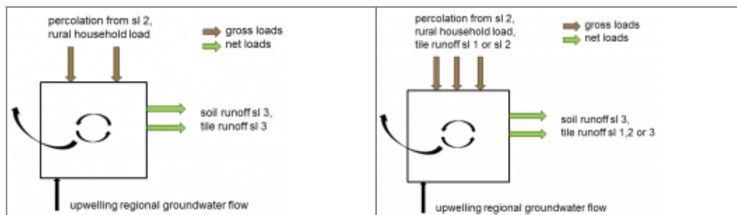
Figure 7: Components of calculated gross (brown) and net (green) loads of soil.
